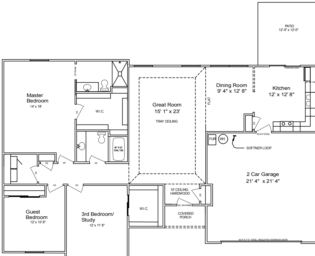
Floor Plan
